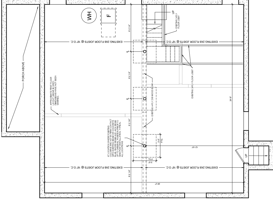
1 BASEMENT PLAN SCALE: 1/4\"/>
