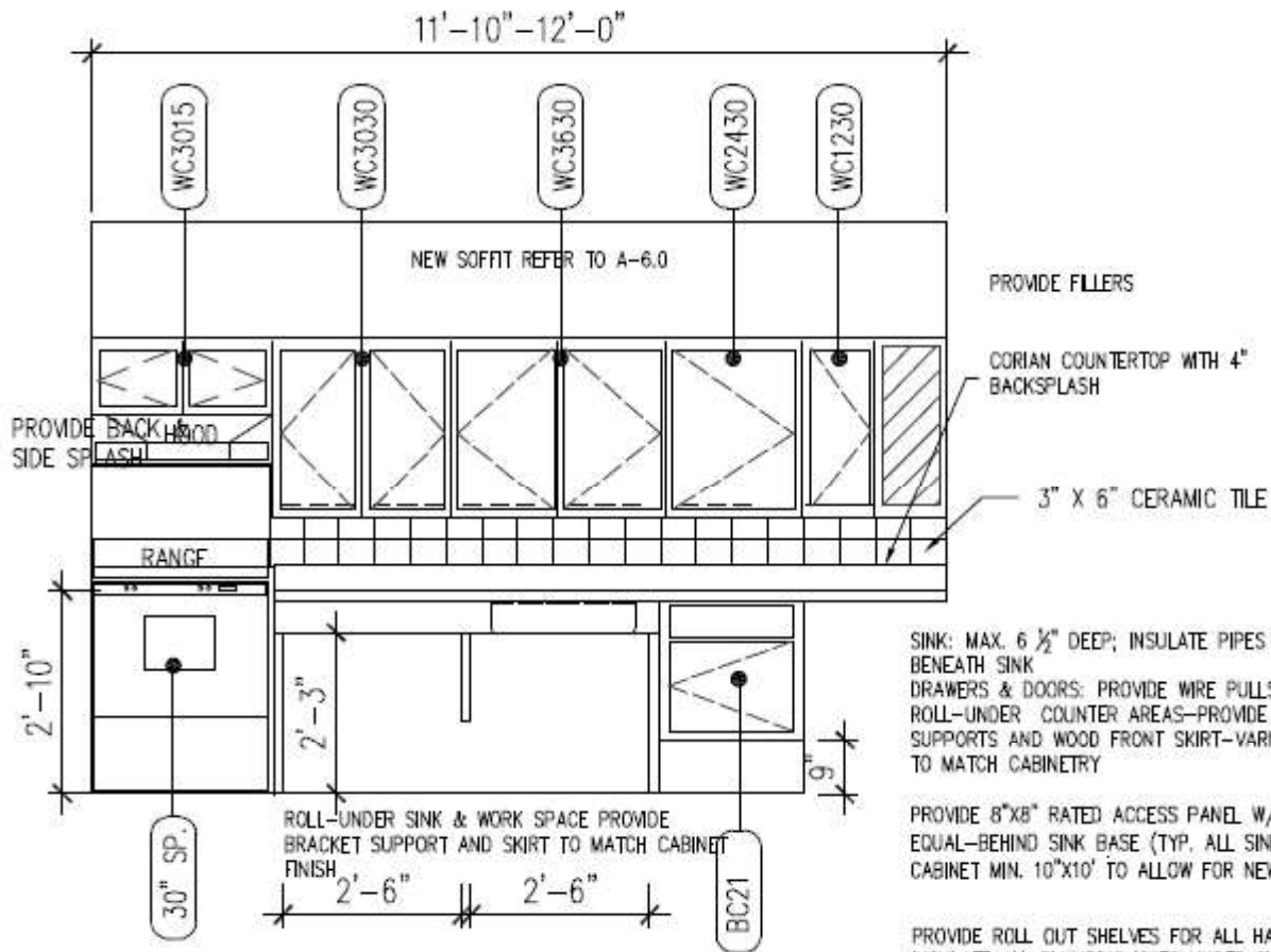
KITCHEN ELEVATION - A
