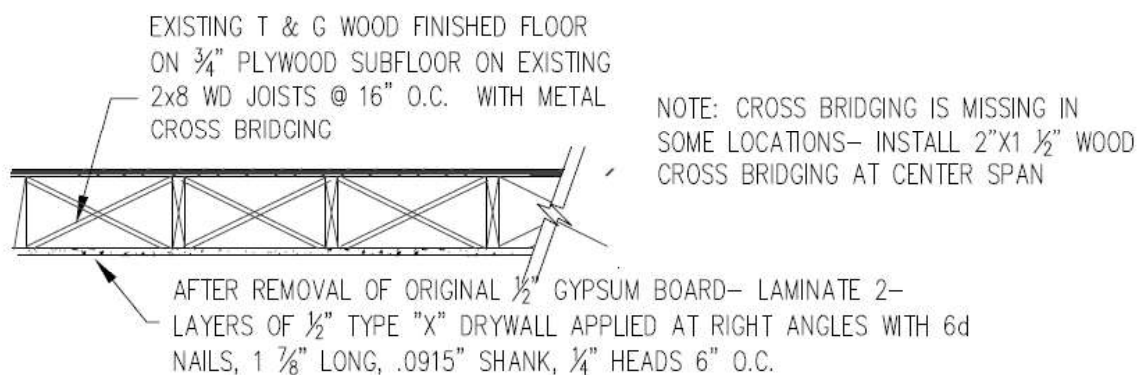
CEILING DETAIL 1
